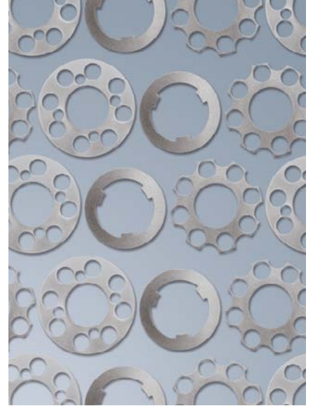
EKagrip® friction shim geometries according to customer specification
